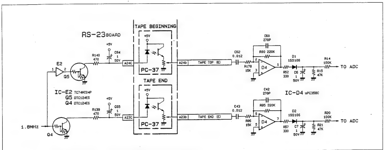
Fig. 4-4-11. Tape Beginning and Tape End Sensors (RS-23 Board)
